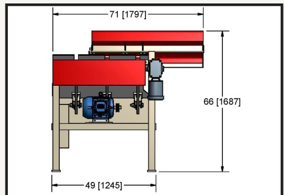
Model OM-3 View of Motor
