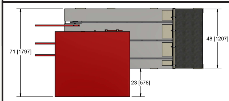
Model OM-2 Top View
