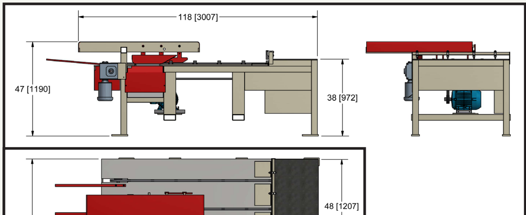
Model OM-2 View of Motor
