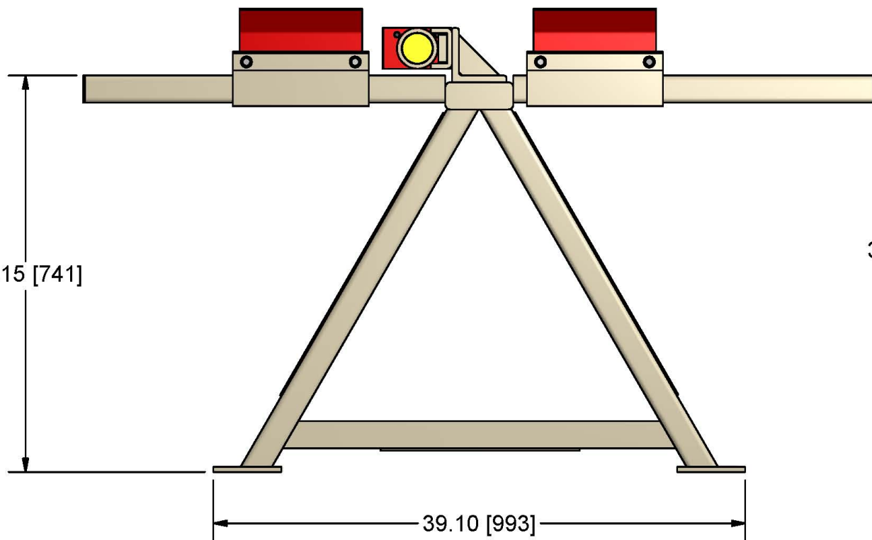
STRINGER-SPLICER
