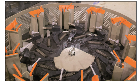
10 x Loading magazines with manual setup
